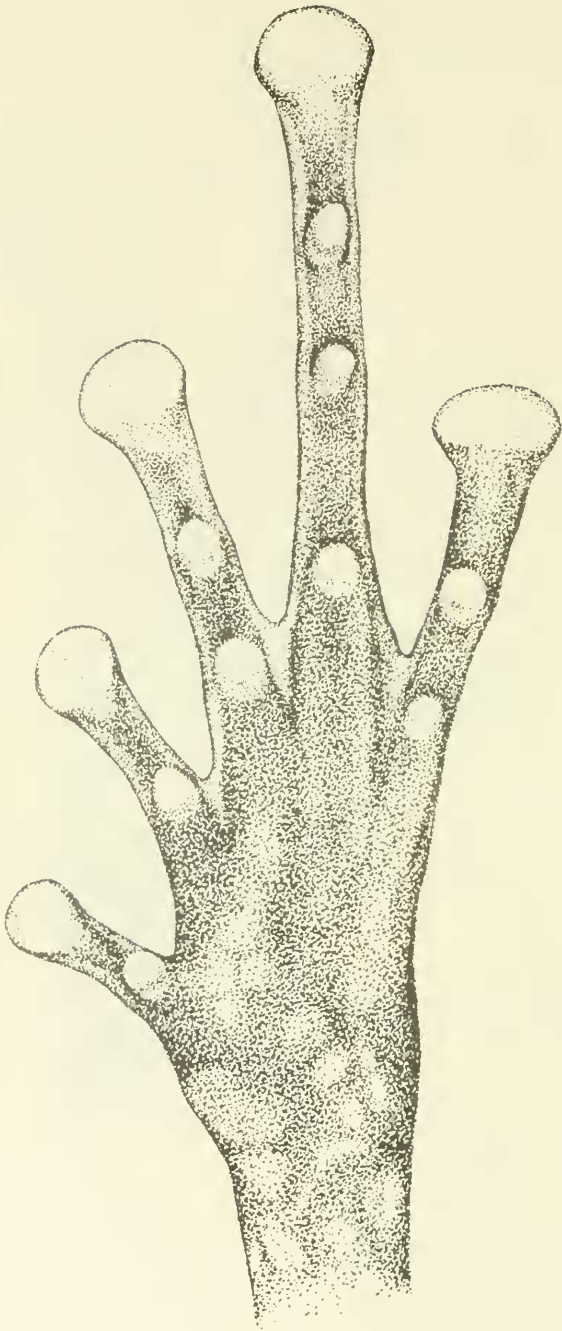
FIGURE 2. Platymantis lawtoni , inferior view of foot.
